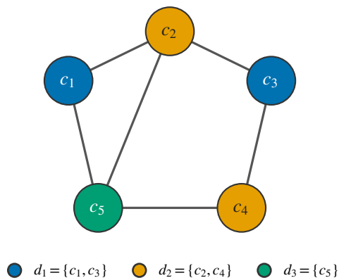
(b) Column-intersection graph G
