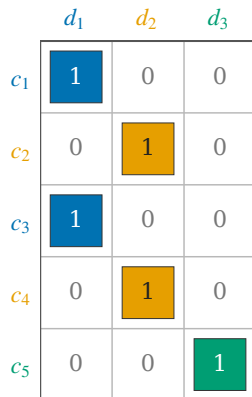
(c) Seed matrix S
