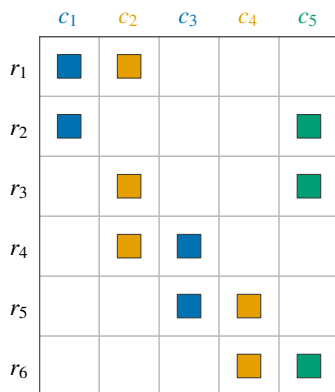
(a) Sparse Jacobian pattern J
