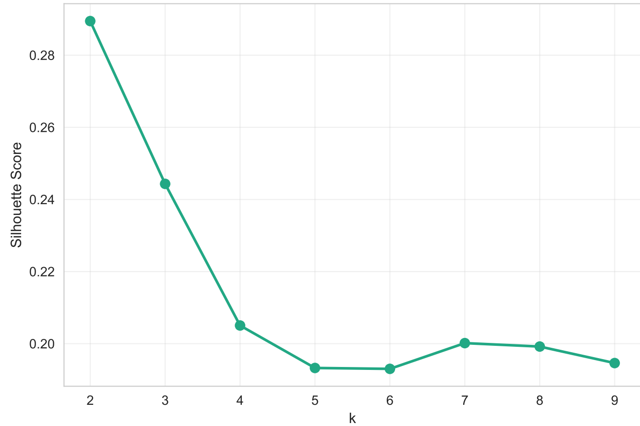
Silhouette Analysis
