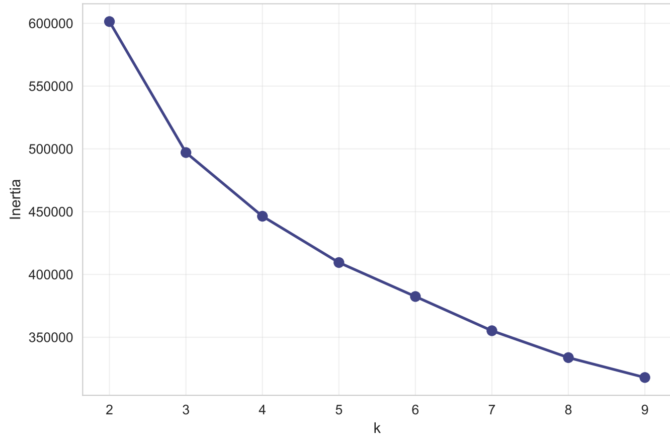
Elbow Method
