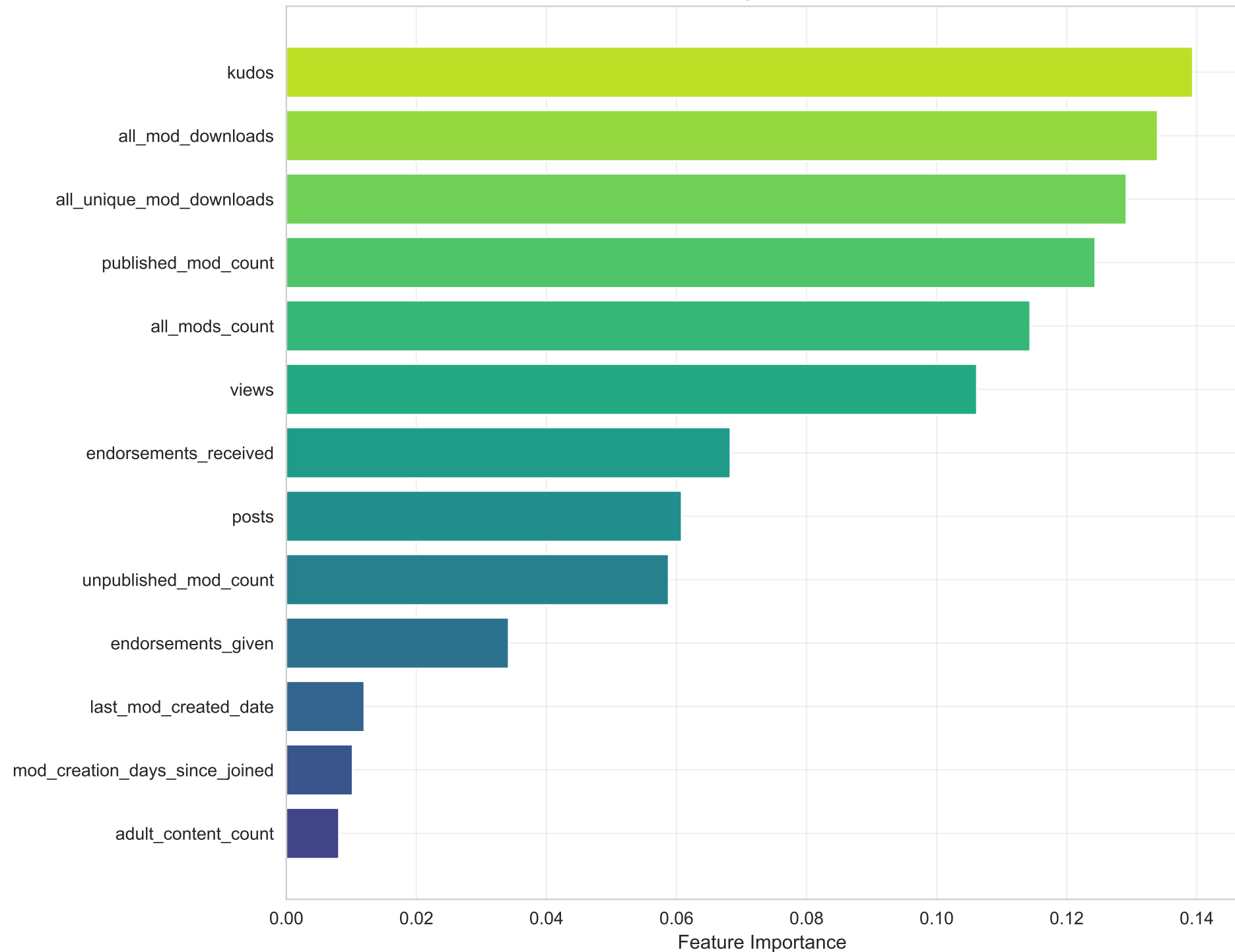
Random Forest Feature Importance for Cluster Prediction
