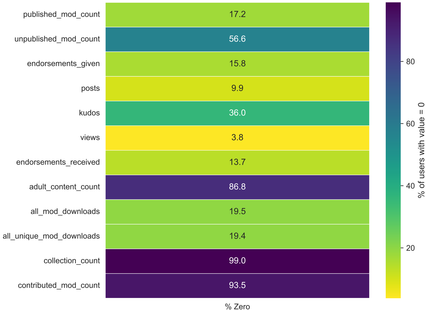
Feature Sparsity Heatmap
