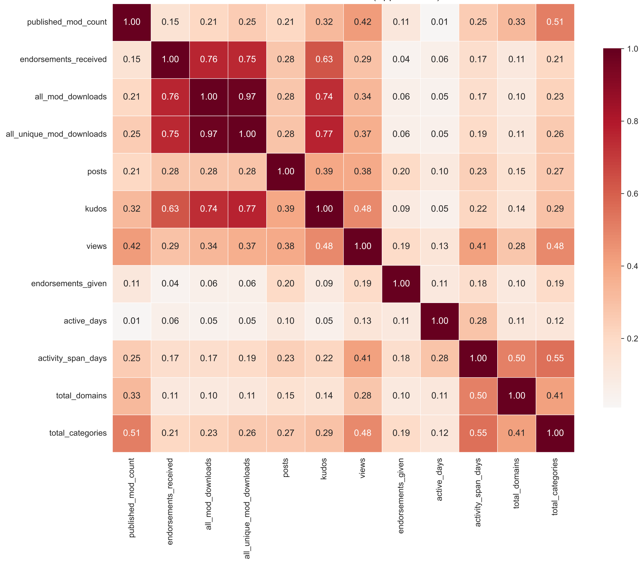
Feature Correlation Matrix (Appendix D6)
