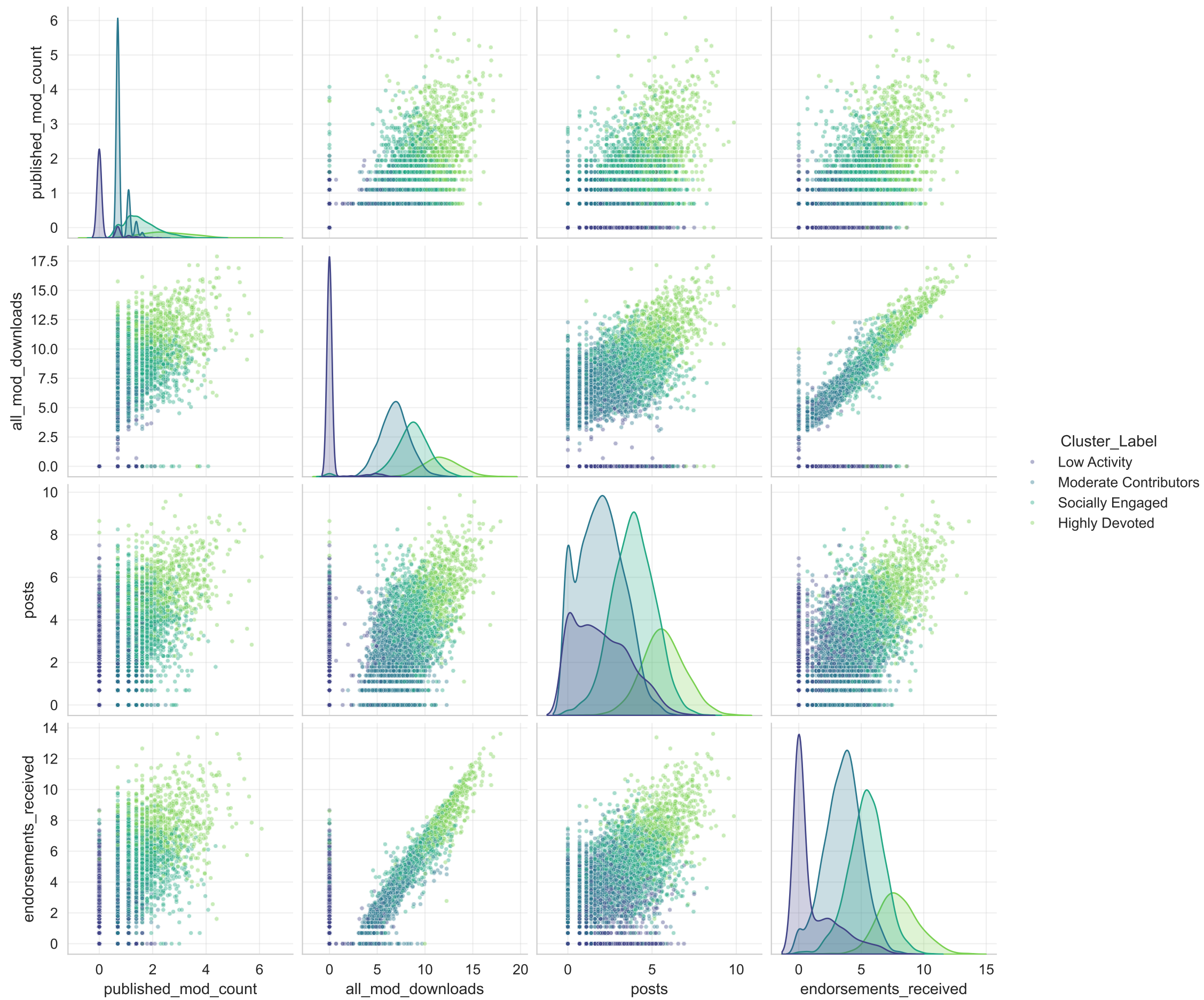
Pairplot of Key Features by Cluster (log scale, N=5000 sample)
