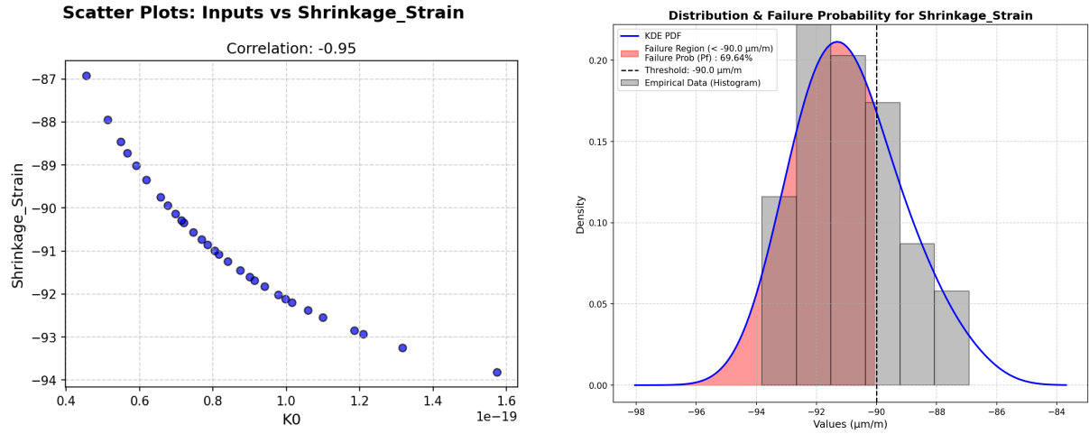
(a) Correlation of K_0 and shrinkage strain.
