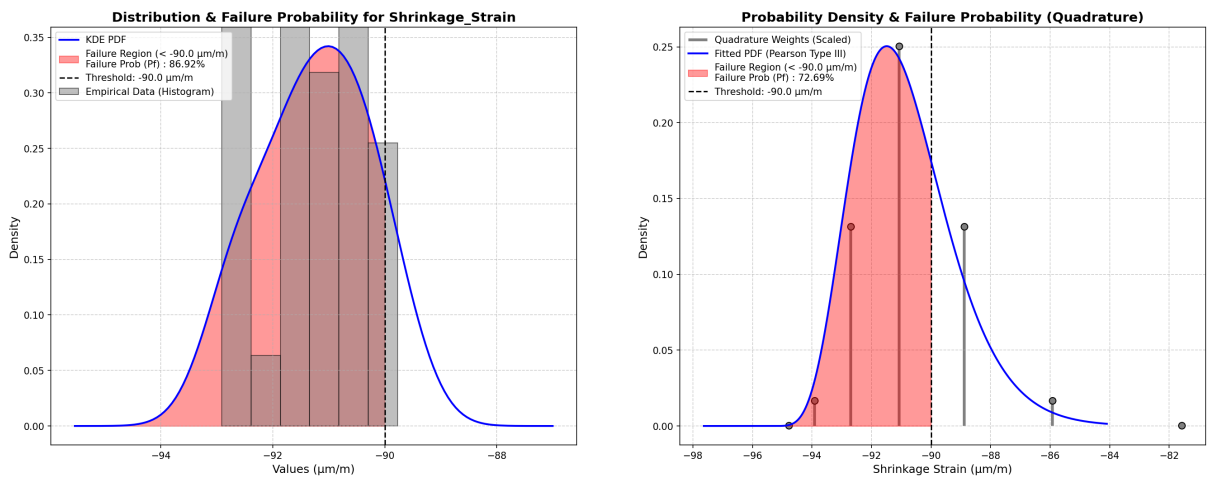
(a) Analysis C2 (Cast3M ALEA).
