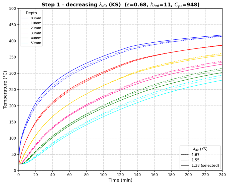
Figure 4.4: Effect of decreasing the conductivity \lambda_{d0} (KS)
