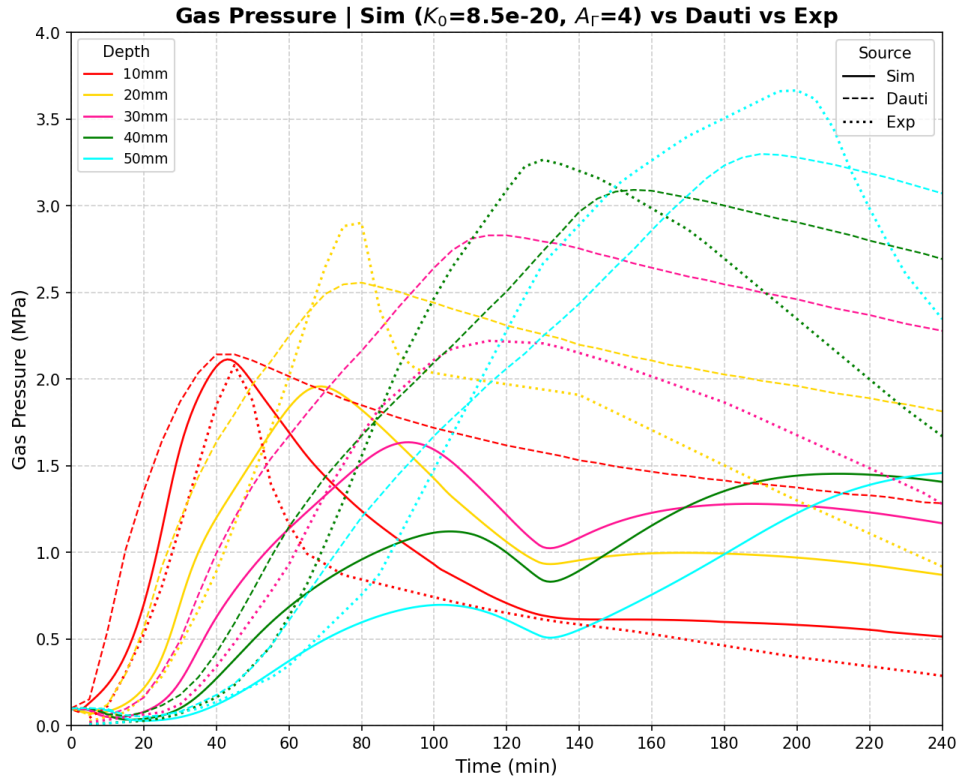
Figure 4.10: Gas pressure with the retained pair ( K_0 = 8.5 \times 10^{-20} \text{ m}^2 , A_r = 4 ): simulation (solid) vs. Dauti (dashed) vs. experiment (dotted)
