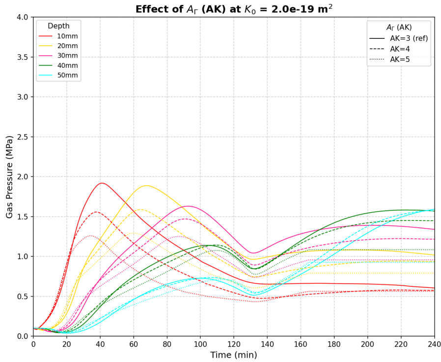
Figure 4.8: Effect of A_\Gamma ( A_K = 3, 4, 5 ) at the initial reference permeability K_0 = 2 \times 10^{-19} \text{ m}^2
