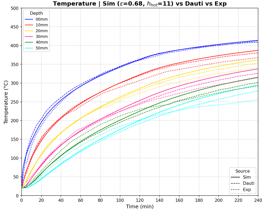
Figure 4.3: Temperature with the reference set ( \varepsilon = 0.68 , h_c = 11 , C_{ps} = 948 , \lambda_{d0} = 1.67 ), compared with the experiment and with Dauti's results.
