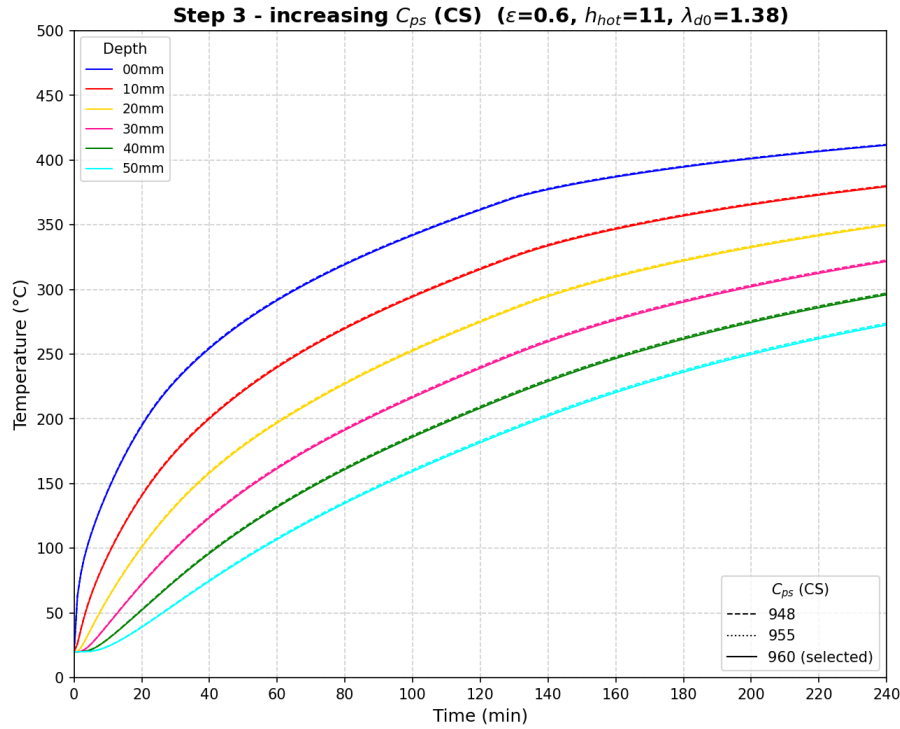
Figure 4.6: Effect of increasing the heat capacity C_{ps} (CS):
