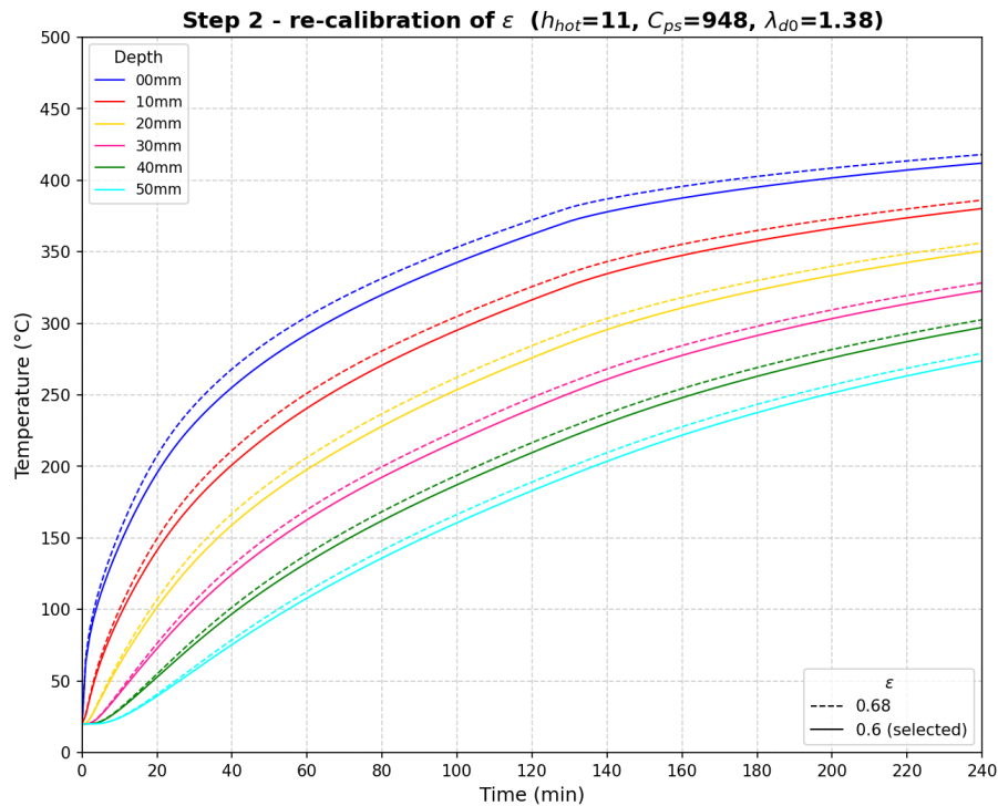
Figure 4.5: Re-calibration of the emissivity \varepsilon after the conductivity was reduced
