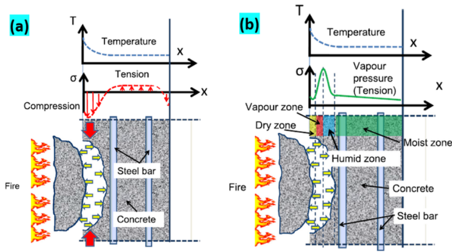
Figure 2.1: Spalling combined mechanisms [aldalaien2025]
