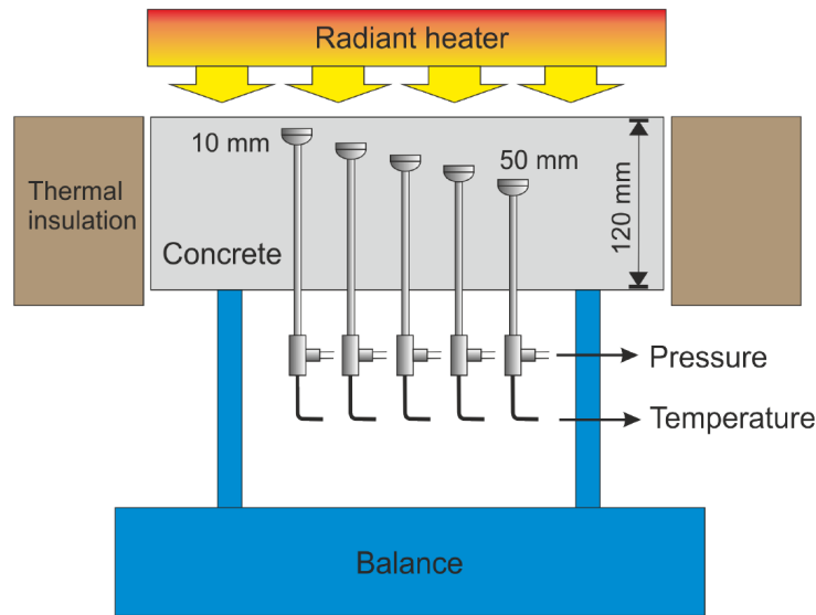
Figure 3.1: Kalifa experiment setup [5]
