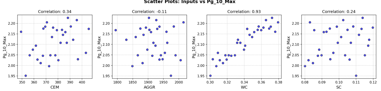
Figure 5.3: Analysis B — correlation: Pearson and Spearman rank correlation of each mix proportion ( c , agg , w/c , s/c ) with the peak pressure p_g^{10} .
