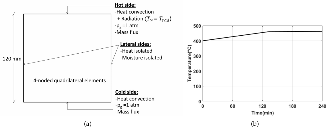
Figure 3.2: (a) Model set-up and boundary conditions and (b) radiator temperature used in the modelling, after Dauti [5].
