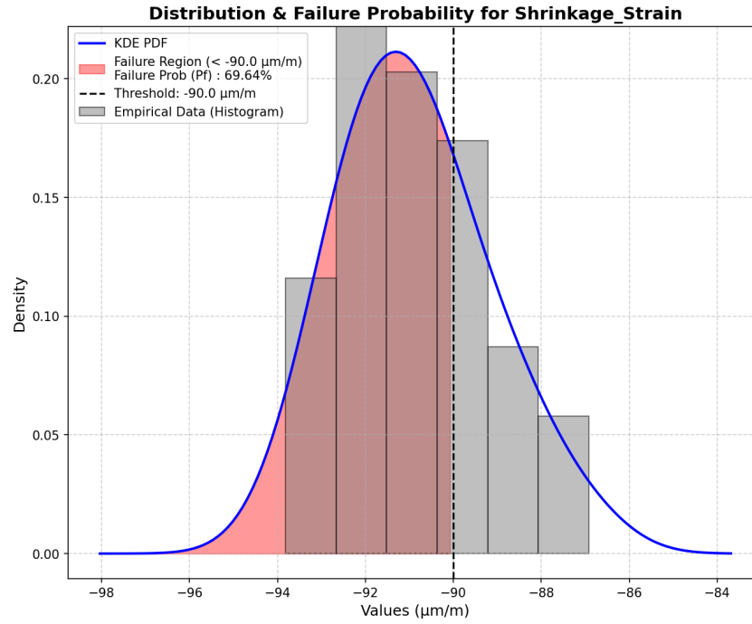
Figure 5.12: Analysis C1 (OpenTURNS + LHS): Probability Density Function (PDF) of the longitudinal shrinkage strain induced by the uncertainty of the intrinsic permeability ( K_0 ).
