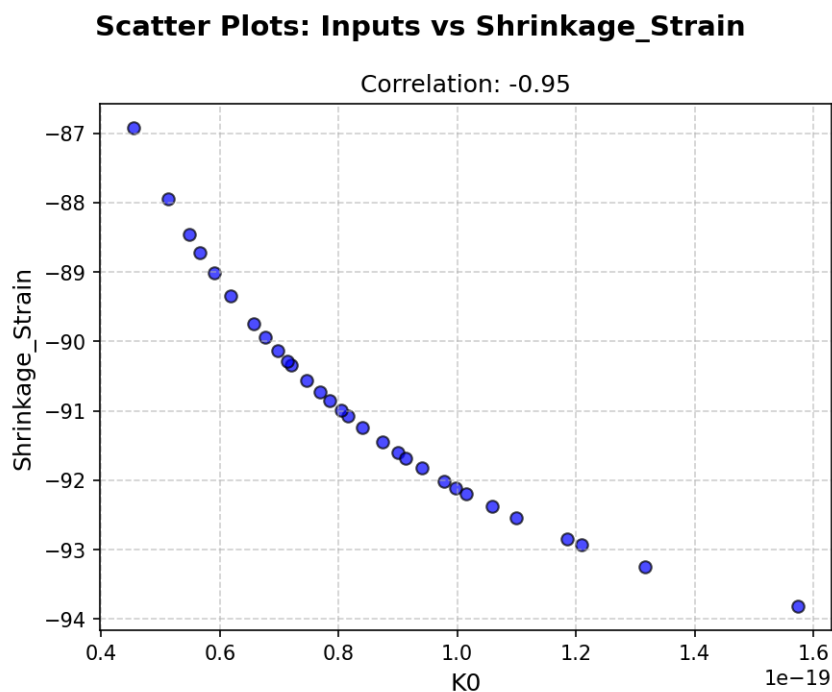
Figure 5.11: Analysis C1 (OpenTURNS + LHS): Pearson and Spearman rank correlation between the intrinsic permeability ( K_0 ) and the resulting longitudinal shrinkage strain.
