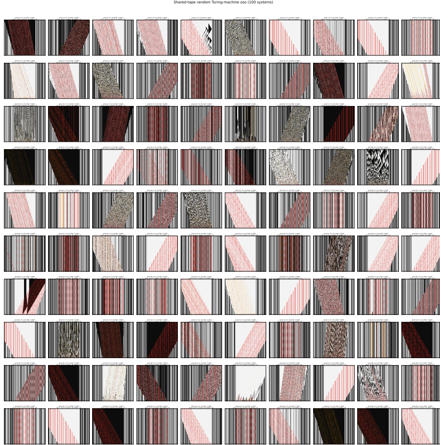
Figure C.3: Three-state reference ensemble: 100 random \text{TM}_3(2) tables, seeds 0–99, with N = 1000 identical copies per panel and q_0^{(i)} = 1 . Each tape starts with independent bits of density p_1 = 1/2 ; heads are spaced five sites apart. Evolution lasts T = 5000 synchronous steps, with majority-vote writes and unchanged symbols on ties. The tape is unbounded and the displayed sites are -5000 \leq x \leq 4999 ; leaving the image does not remove a head. Snapshots were recorded every five steps. This is the reference for the additional seeds, blank tape, and asynchronous comparisons below. Time runs upward; dark/light denotes V = 0/1 , and red/yellow denotes single/multiple heads.
