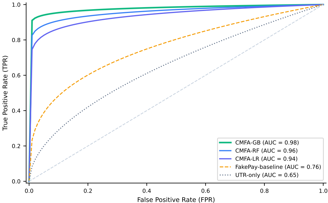
ROC Curves Comparison
