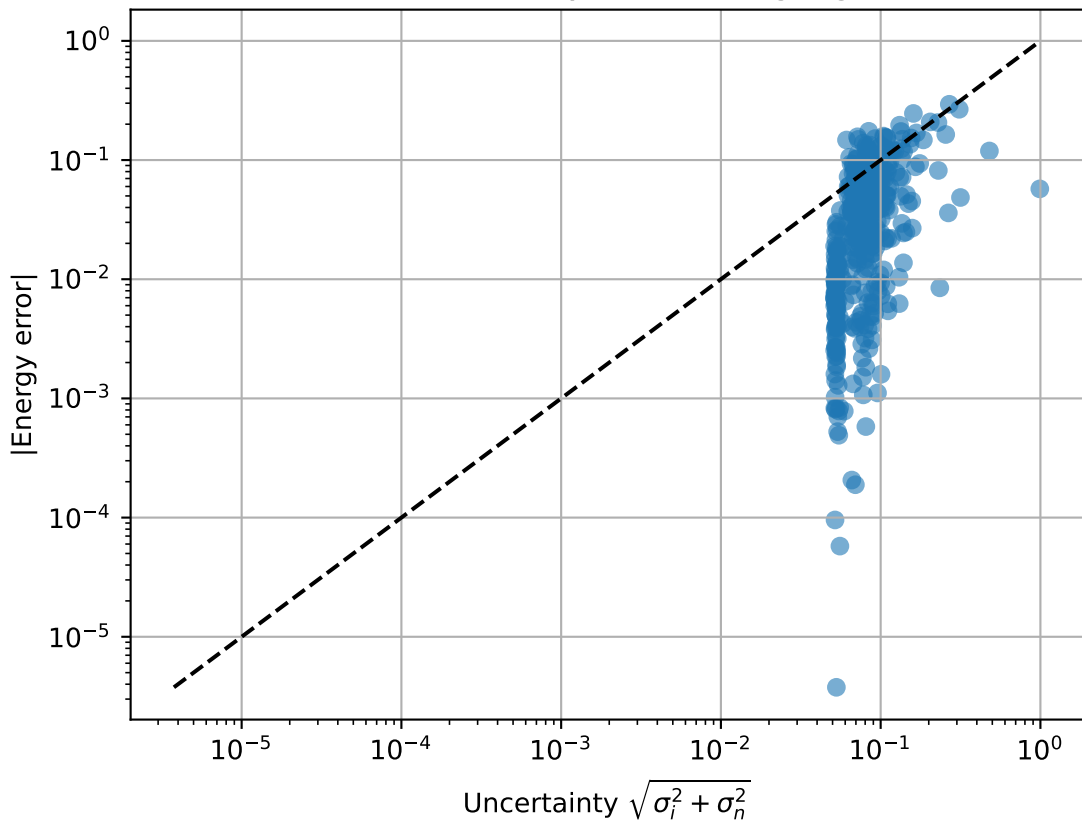
GP uncertainty vs error (log-log)
