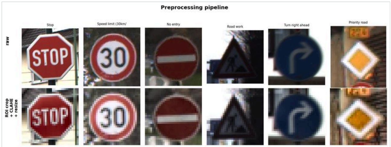
Figure 3. The preprocessing pipeline. Top row: raw images as recorded, with background and uneven exposure. Bottom row: after ROI crop, CLAHE and resize to 32 \times 32 . Contrast is normalised across very different lighting conditions while colour is preserved.
