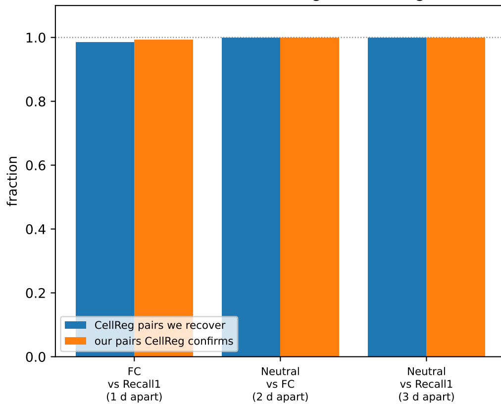
Ca-EEG2-1: matcher against CellReg
