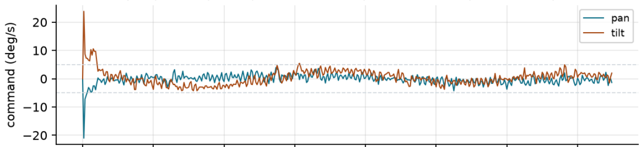
Platform sway 12 px/frame plus 20 px/frame vibration: gimbal command against the 5 deg/s limit
