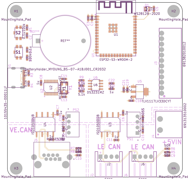
Top Assembly (Scale 1:1)
