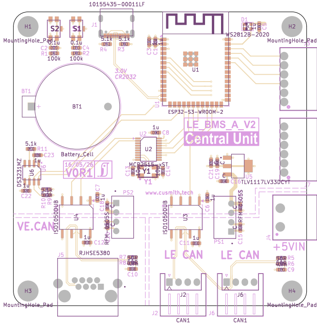
Top Assembly (Scale 1:1)
