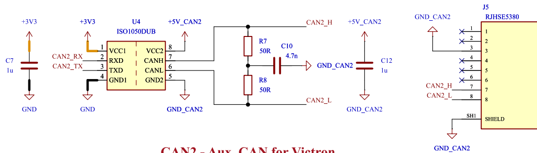
CAN2 - Aux. CAN for Victron
