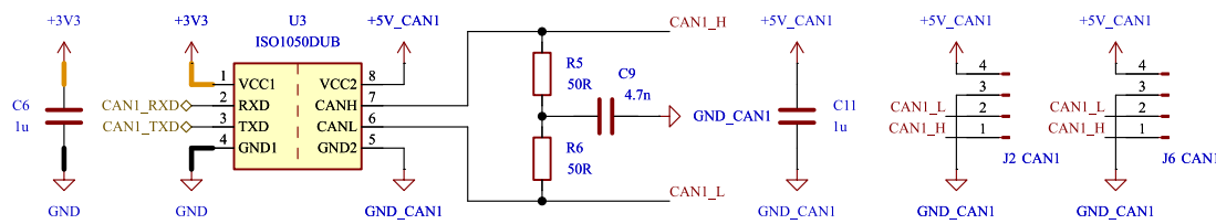
CAN1 - Native ESP32
