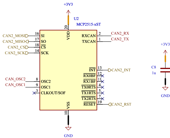
SPI CAN Interface
