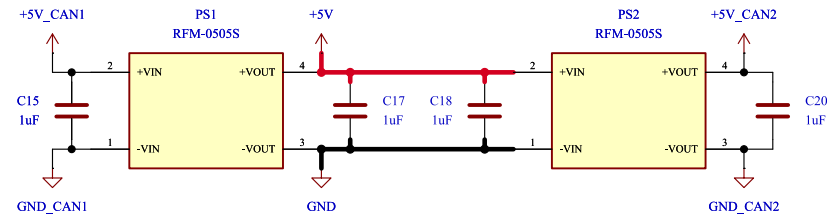
5V and 5V_CAN2 Generation
