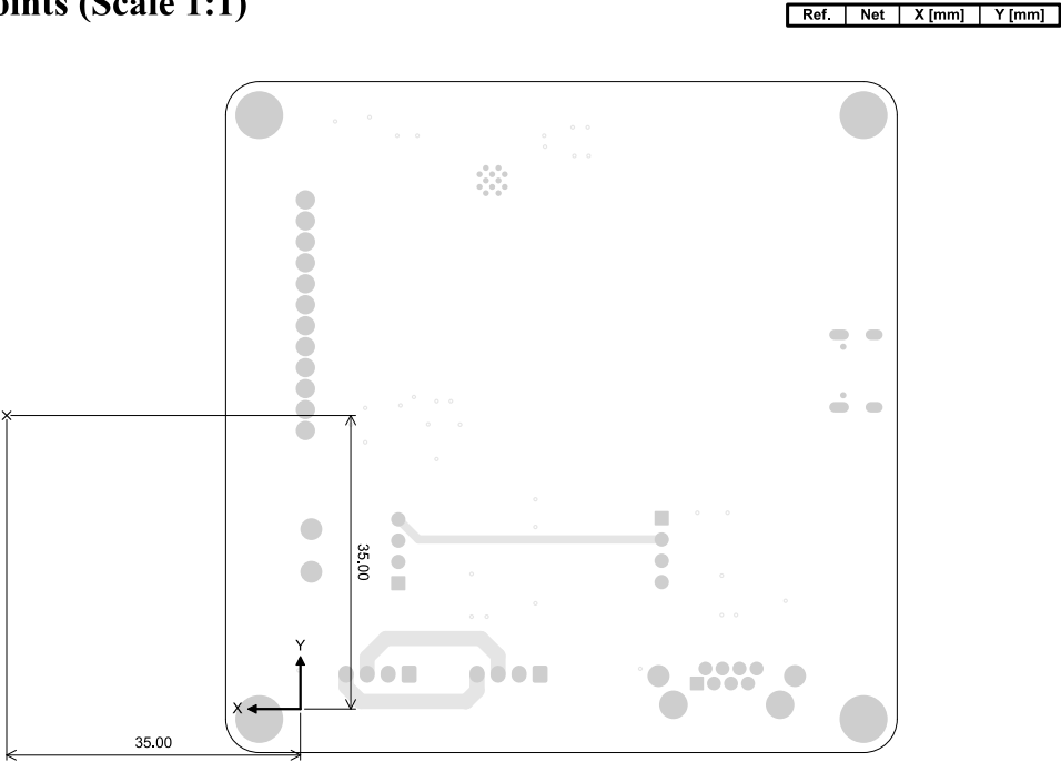
Bottom Test Points (Scale 1:1)
