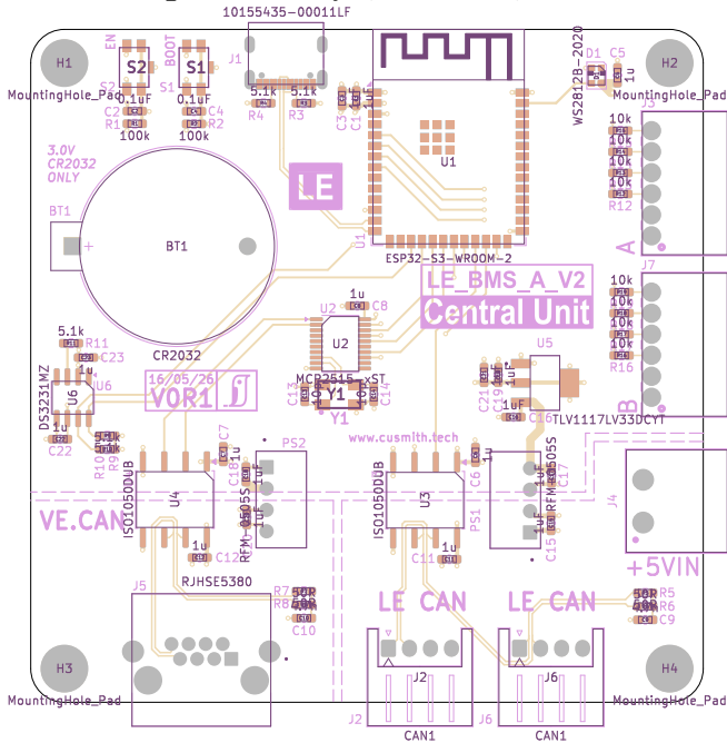
Top Assembly (Scale 1:1)
