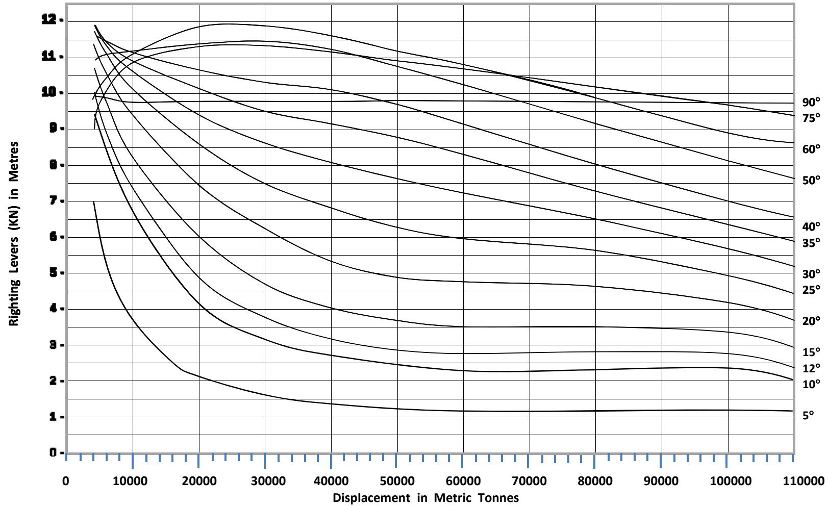
Cross Curves of Stability (KN Curves)
