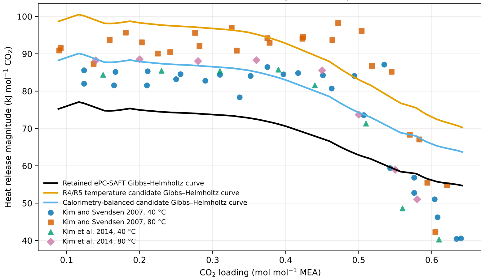
30 wt% MEA calorimetry consistency
