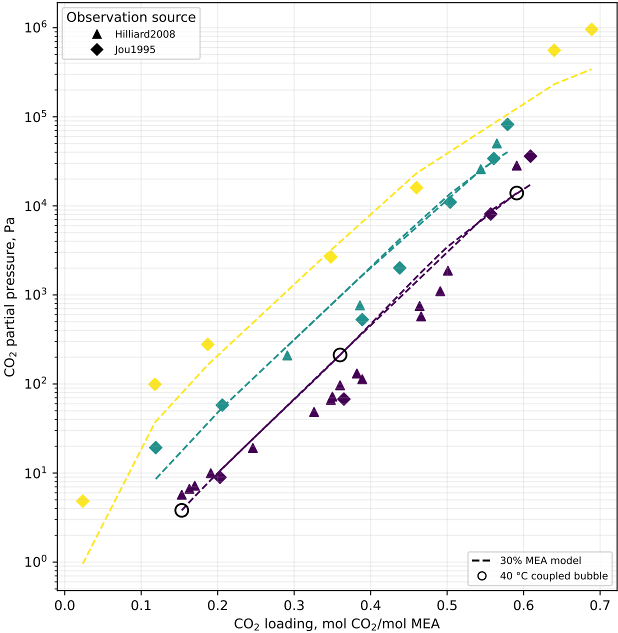
30 wt% MEA pressure block
