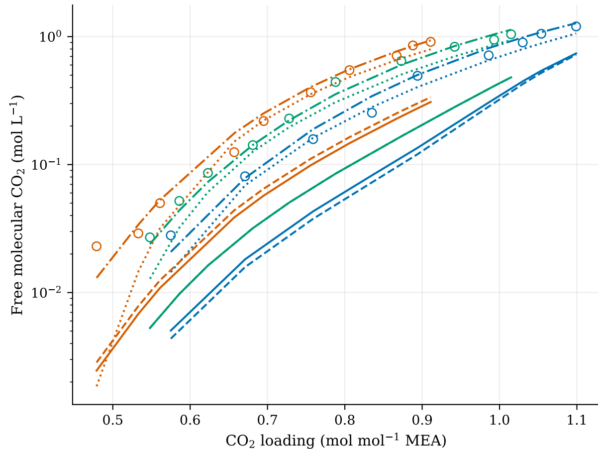
Wong et al. (2016) 30 wt% MEA free-CO 2 external challenge RMS concentration factor: retained 3.79, balanced 3.74, R4 candidate 1.74, CO 2 -water candidate 1.19
