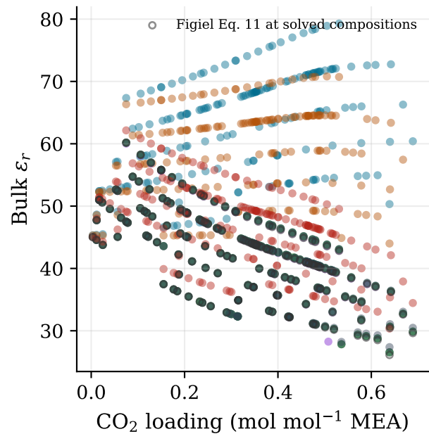
Permittivity response
