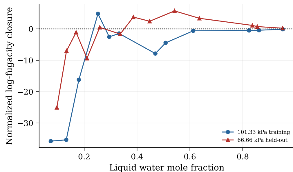
Baygi 3B/4C: MEA closure, k_{ij} = -0.01002
