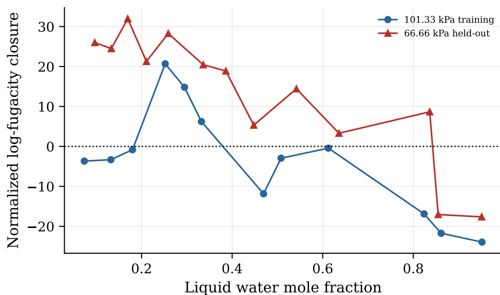
Baygi 3B/4C: Water closure, k_{ij} = -0.01002
