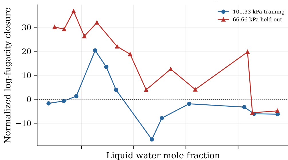
Baygi 3B/4C: Water closure, k_{ij} = -0.01002
