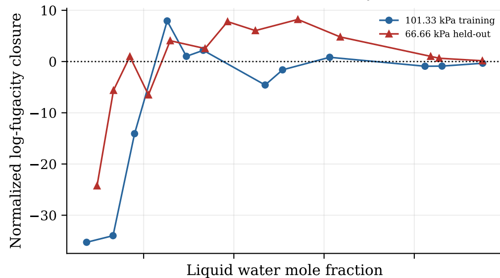
Baygi 3B/4C: MEA closure, k_{ij} = -0.01002
