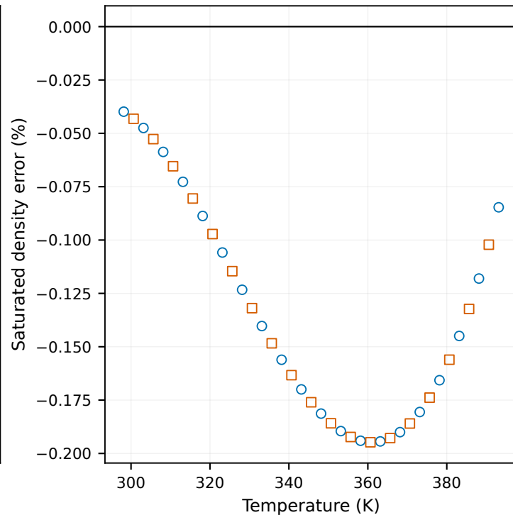
Saturated liquid density
