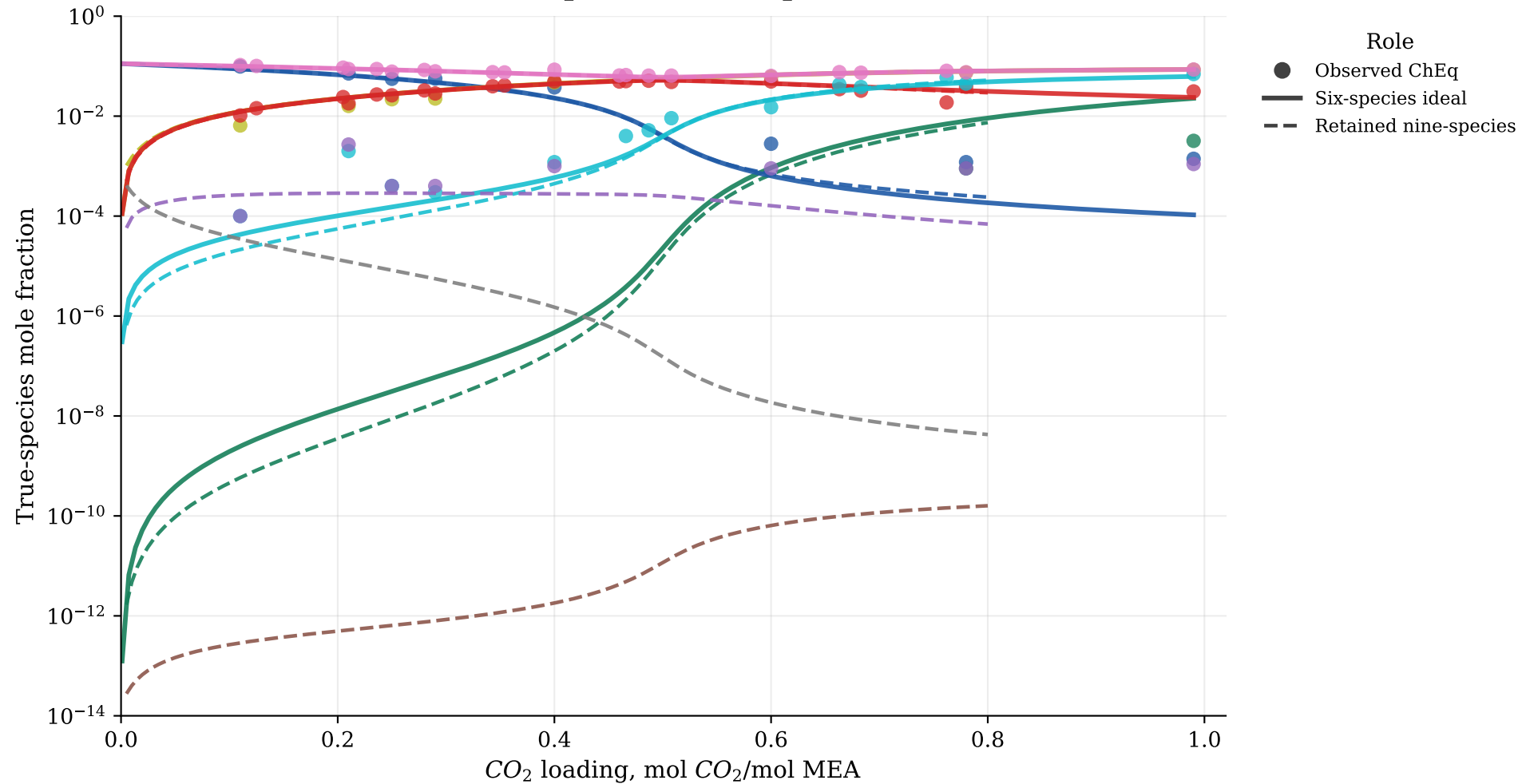
30 wt% MEA speciation comparison, 40 °C
