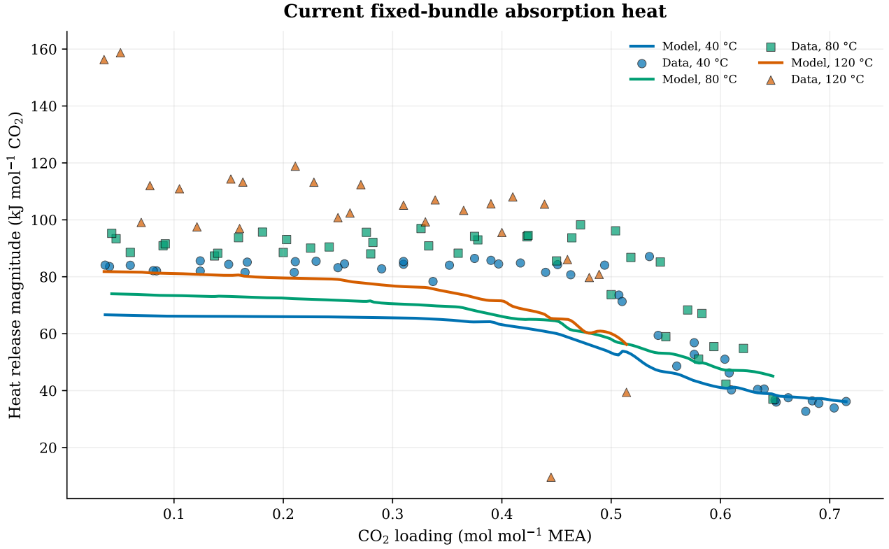
Figure 1: Retained calorimetry observations (points) and the current fixed Tables 1–4 bundle evaluated by direct total reactive enthalpy (continuous lines). Lines are shape-preserving interpolations of the scored finite-interval predictions; no calorimetry parameter was fitted.
