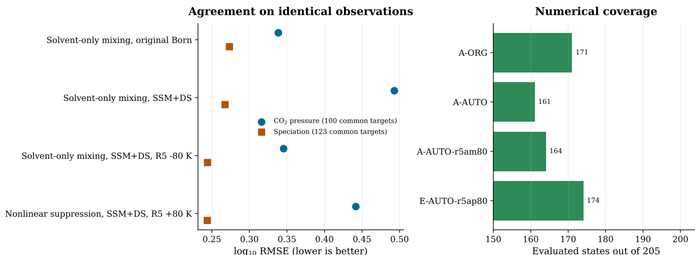
Figure 4: Current reaction-synchronized comparison. Pressure and speciation \log_{10} RMSE use observations evaluated by all four configurations ( n_p = 100 , n_x = 123 ); the right panel reports all successful states out of 205 attempts. Lower RMSE is better.
