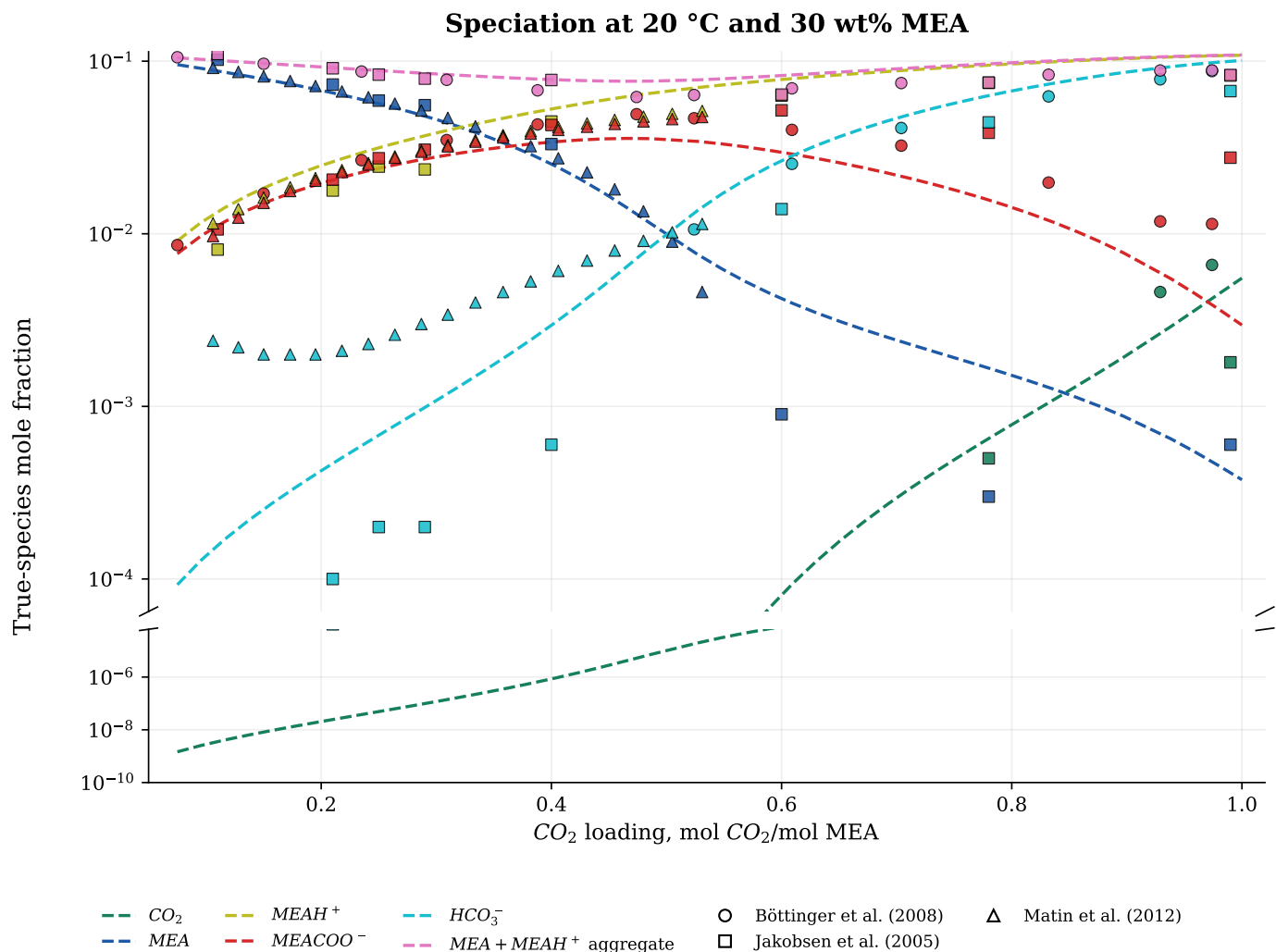
Figure 1. Current smooth-grid diagnostic for the full nine-species liquid-equilibrium replay at 20 °C and 30 wt% MEA. Symbols show all positive retained Böttinger, Jakobsen, and Matin values for the displayed series; symbol shape identifies source and color identifies species. The broken logarithmic axis expands the 5.6248 \times 10^{-5} – 0.1134 principal-species region and compresses the 10^{-10} – 5.6248 \times 10^{-5} range. Dashed lines connect direct Engine evaluations of the selected bundle through loading 1.0.
