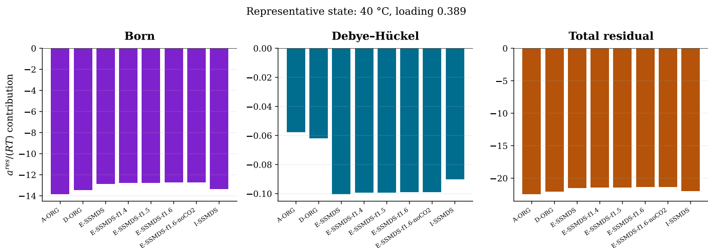
Figure 8: Born, Debye-Hückel, and total residual Helmholtz contributions at one common representative state. Each panel has its own ordinate scale.
