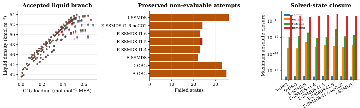
Figure 7: Accepted liquid density, preserved failure classes, and maximum charge, material, reaction-affinity, and pressure closure for every promoted configuration.
