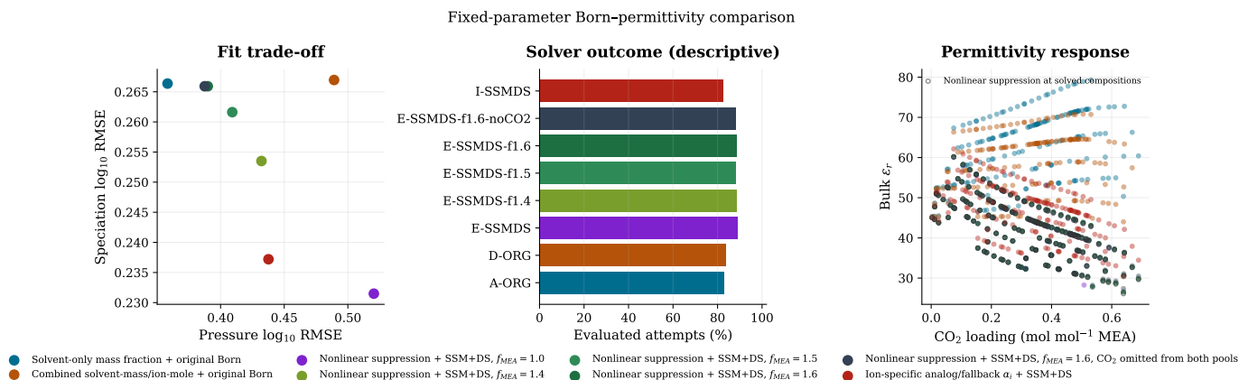
Figure 3: Fixed-parameter trade-off, descriptive evaluated-attempt fraction, and bulk relative permittivity for every promoted configuration. The open circles apply the nonlinear ionic-suppression equation to solvent-only-mass-fraction/original- Born solved compositions; they are a crossover, not independent loaded-MEA dielectric observations. Attempt fraction is not used to rank formulations.
