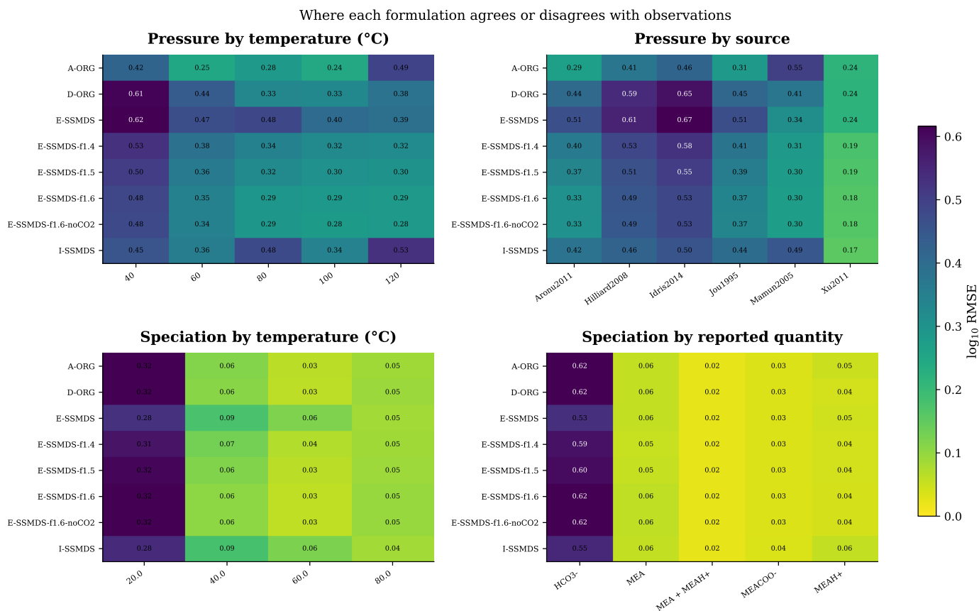
Figure 6: Log 10 RMSE grouped by pressure temperature and source, and by speciation temperature and reported quantity. Missing groups remain missing rather than being imputed.
