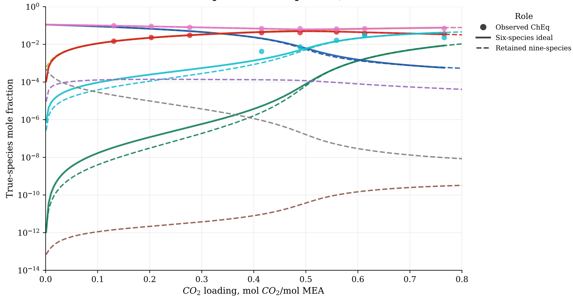
30 wt% MEA speciation comparison, 60 °C
