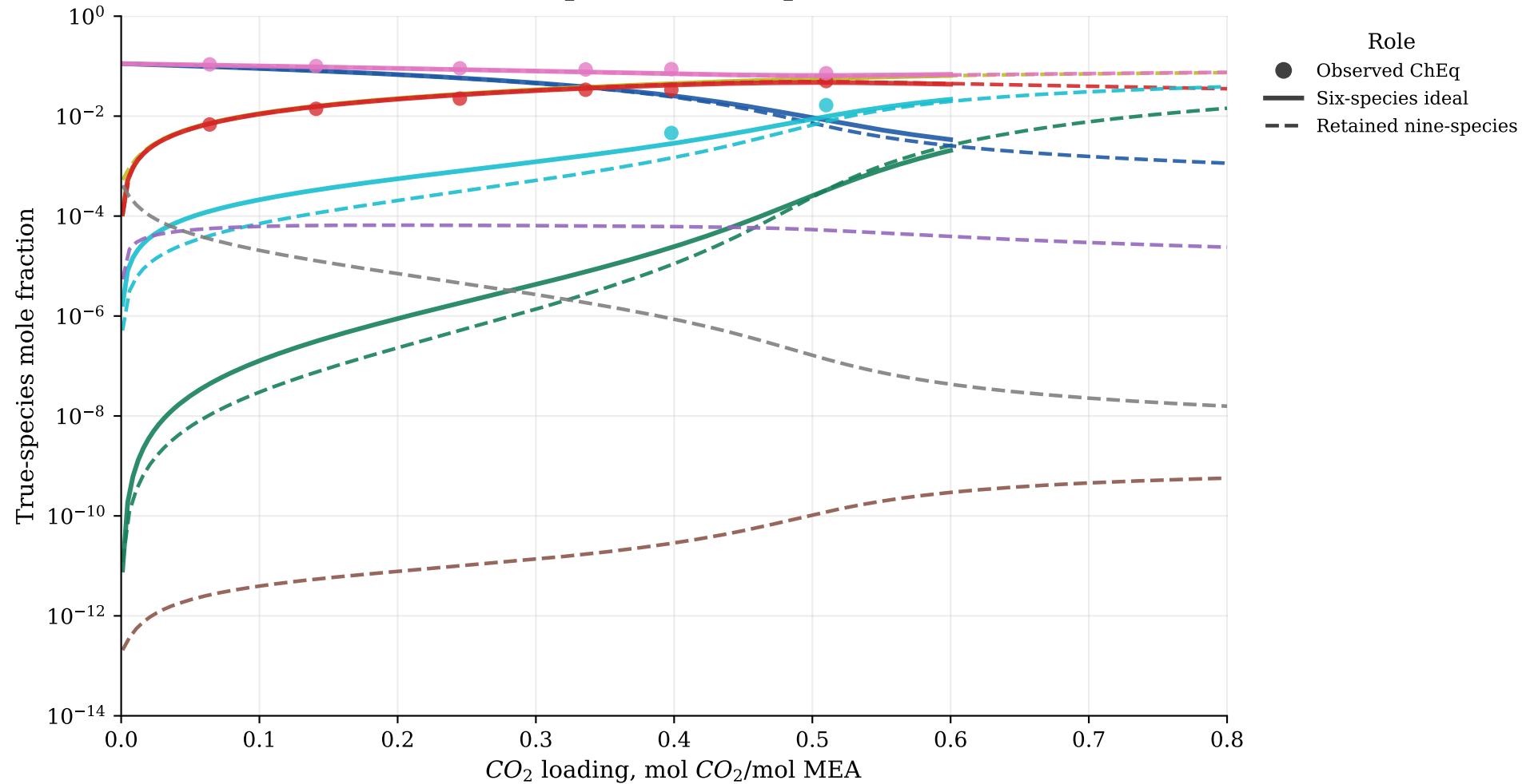
30 wt% MEA speciation comparison, 80 °C
