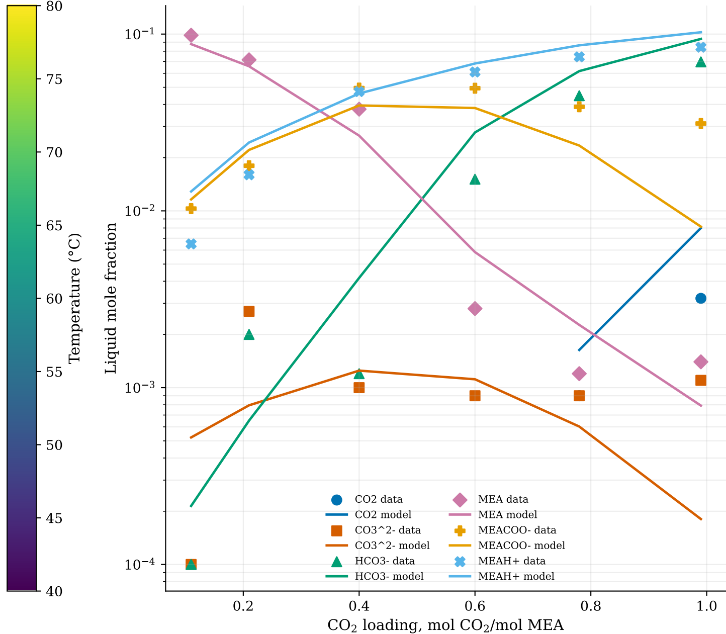
Direct Jakobsen speciation block, 40 °C
