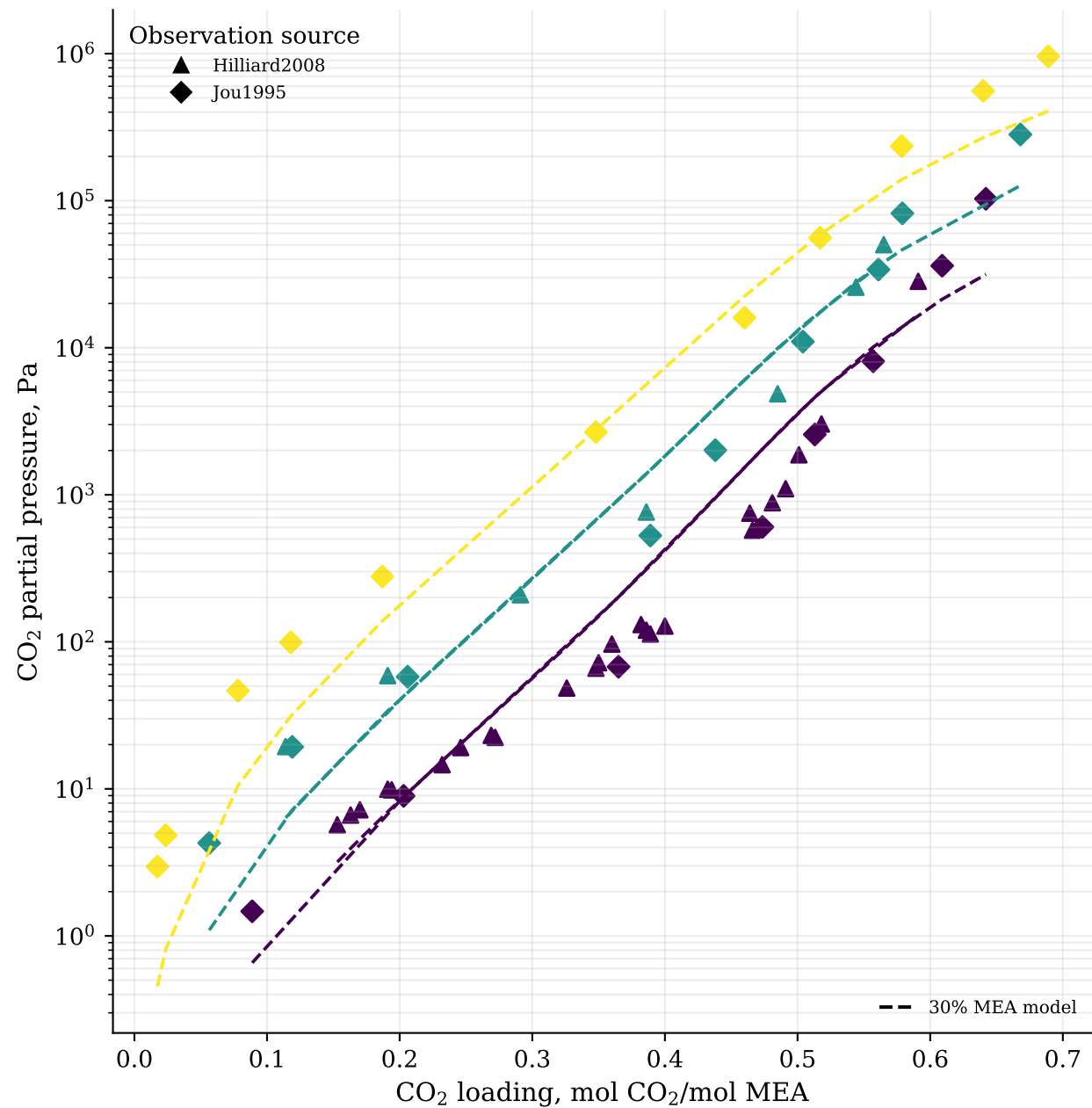
30 wt% MEA pressure block
