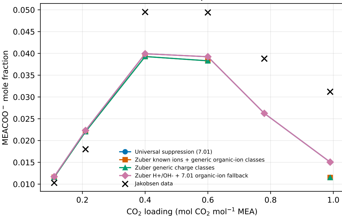
Carbamate speciation
