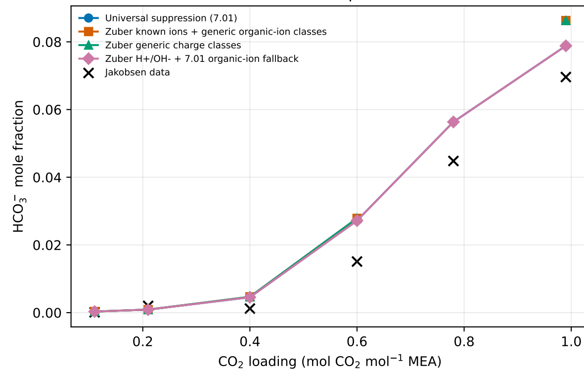
Bicarbonate speciation
