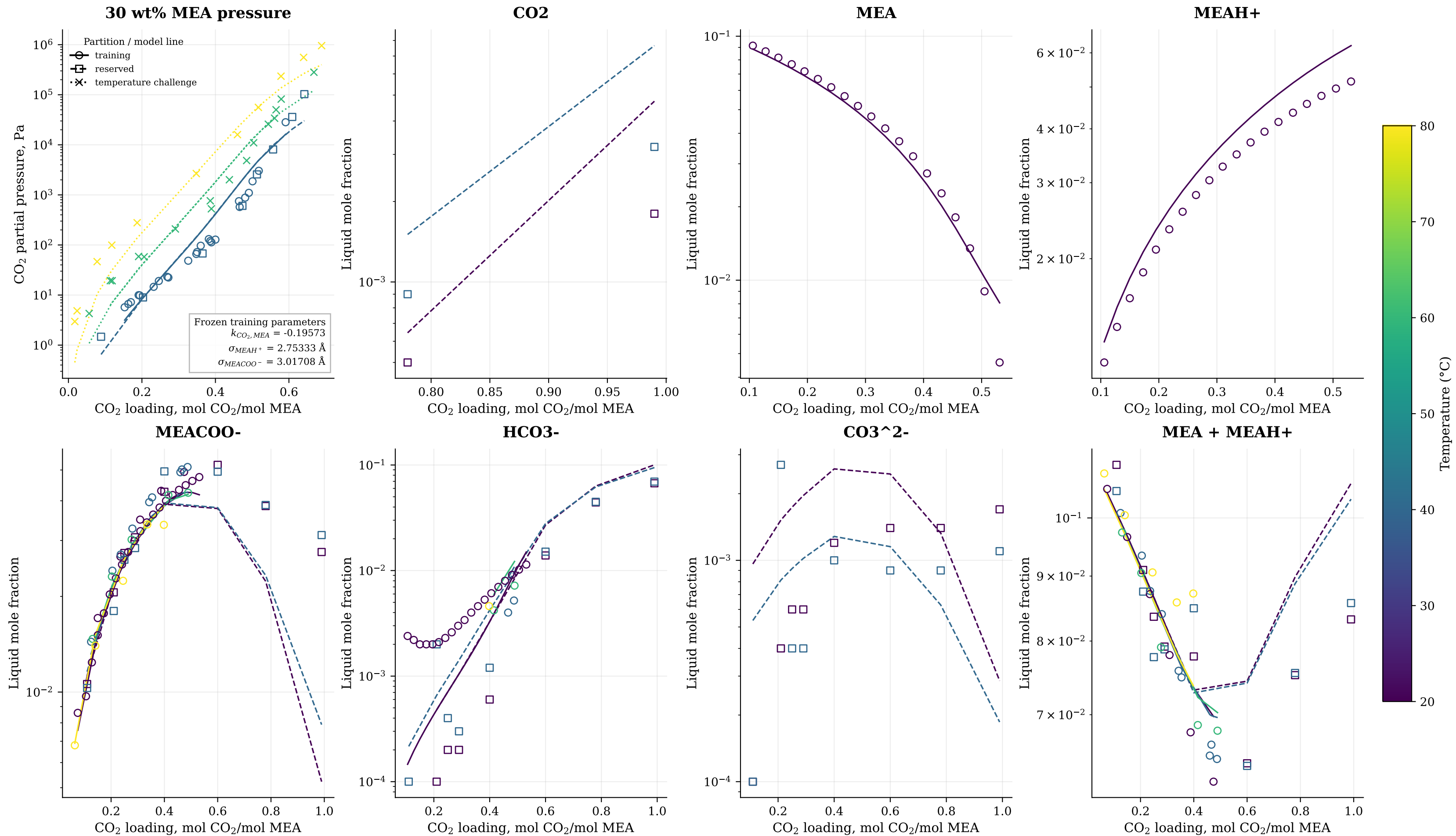
Frozen MEA parameter prediction: training, untouched reserved data, and temperature challenge
