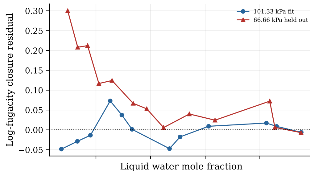
Held water + 4C MEA: Water closure, k_{ij} = -0.03627
