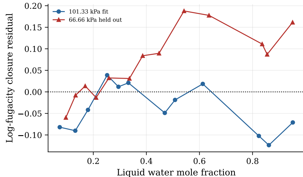
Held water + 4C MEA: MEA closure, k_{ij} = -0.03627
