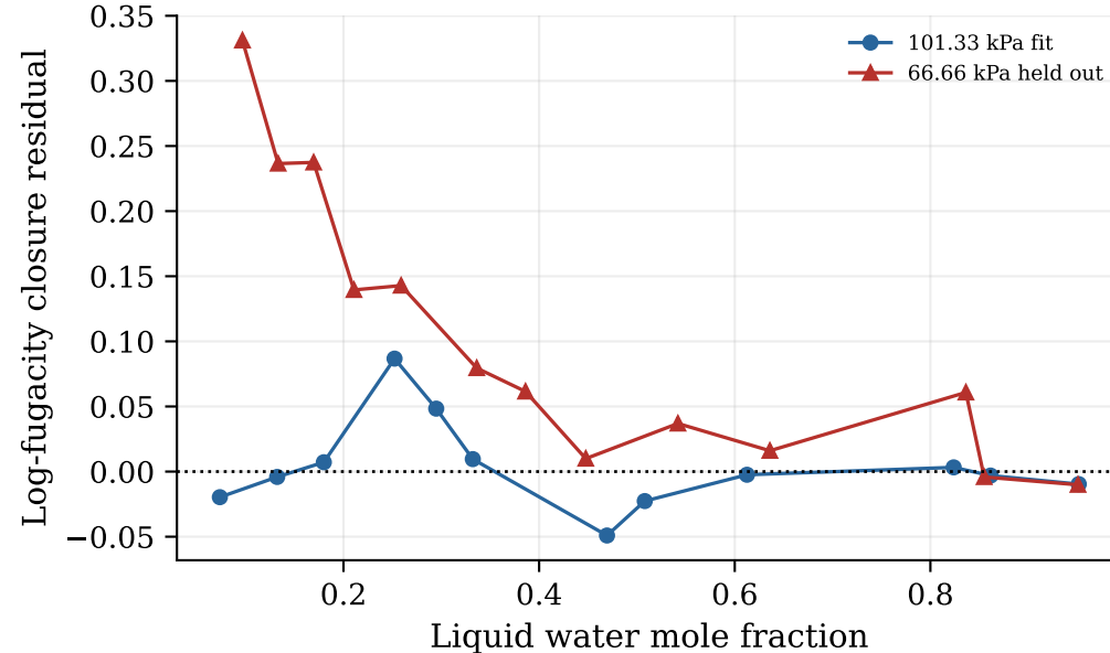
Held water + 4C MEA: Water closure, k_{ij} = -0.03627
