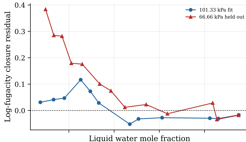
Held water + 3B MEA: Water closure, k_{ij} = -0.01957
