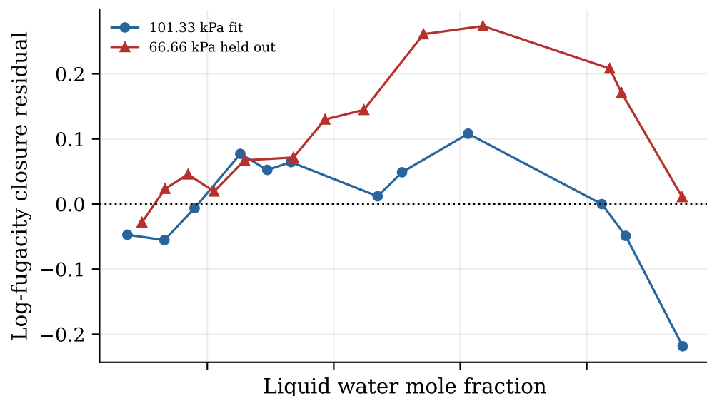
Held water + 3B MEA: MEA closure, k_{ij} = -0.01957
