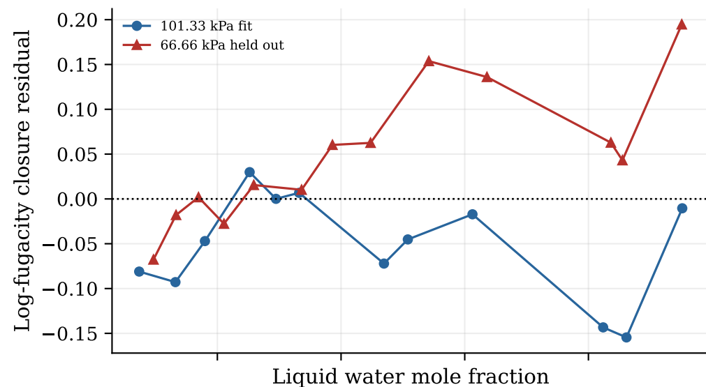
Held water + 4C MEA: MEA closure, k_{ij} = -0.03627
