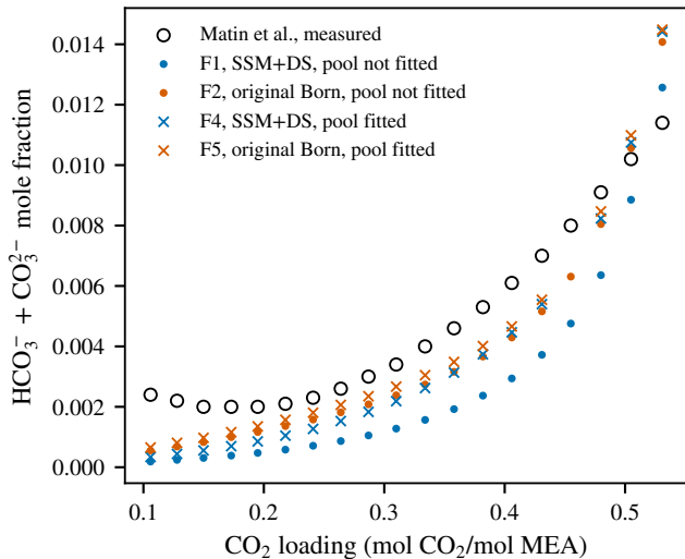
(a) Titration bicarbonate pool, 20 °C
