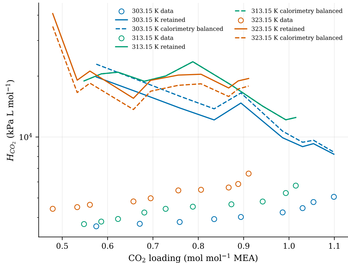
Wong et al. (2016) 30 wt% MEA free-CO 2 external challenge RMS concentration factor: retained 3.79, balanced 3.74
