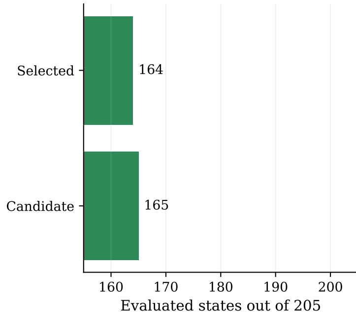
Numerical coverage
