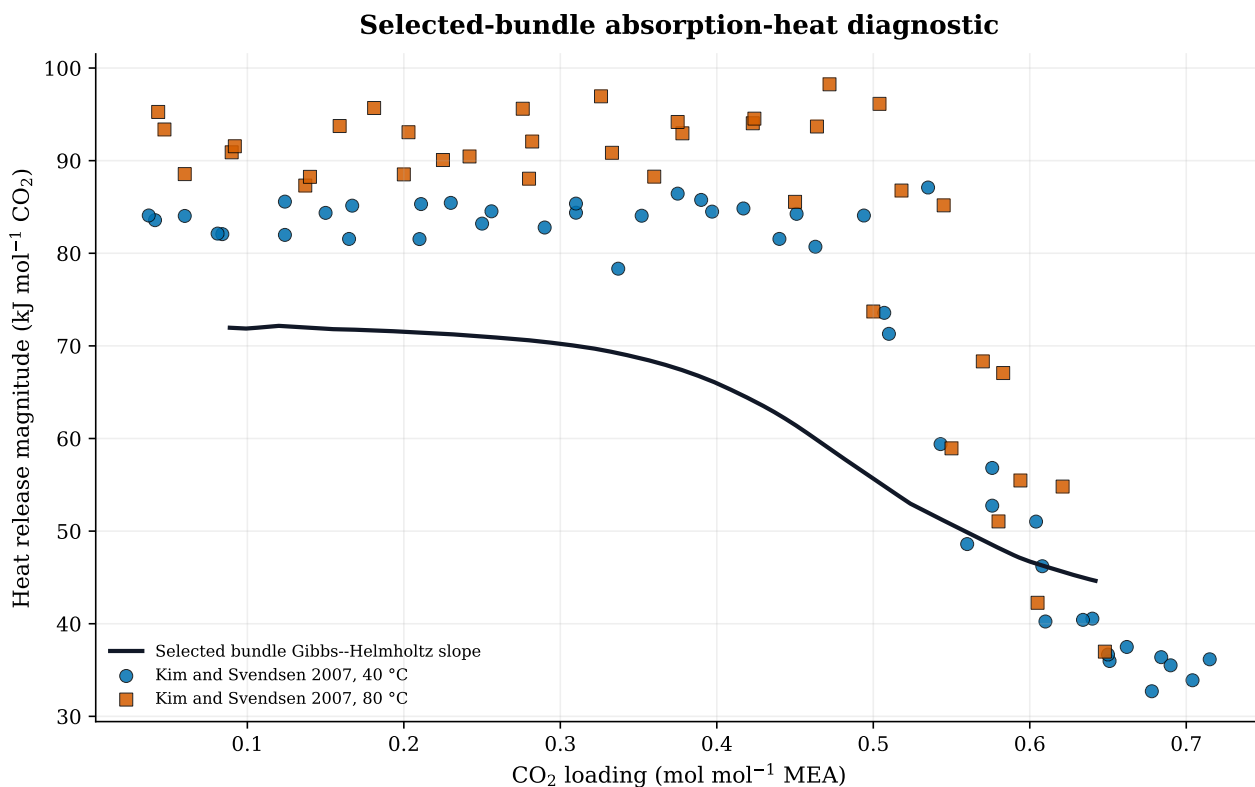
Figure 1: Retained direct calorimetry observations and the selected bundle’s Gibbs–Helmholtz pressure-slope diagnostic. Points are measurements; the line is calculated from the same active Tables 1–4 bundle used for the pressure and speciation figures.
