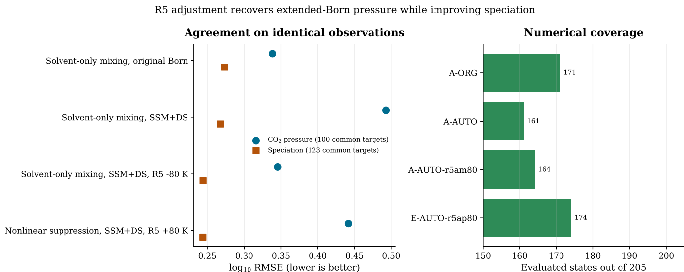
Figure 4: Current reaction-synchronized comparison. Pressure and speciation \log_{10} RMSE use observations evaluated by all four configurations ( n_p = 100 , n_x = 123 ); the right panel reports all successful states out of 205 attempts. Lower RMSE is better.
