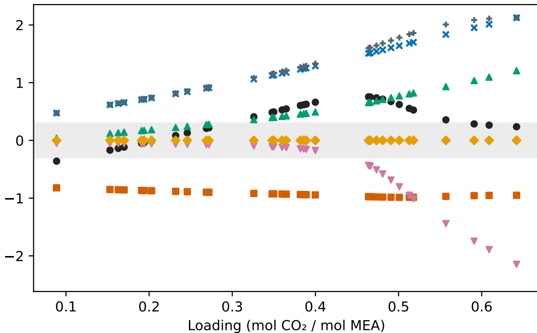
Born-off activity-sum shifts exceed speciation shifts Pipeline verification on pre-#152 data; method development, not manuscript values 313.15 K
