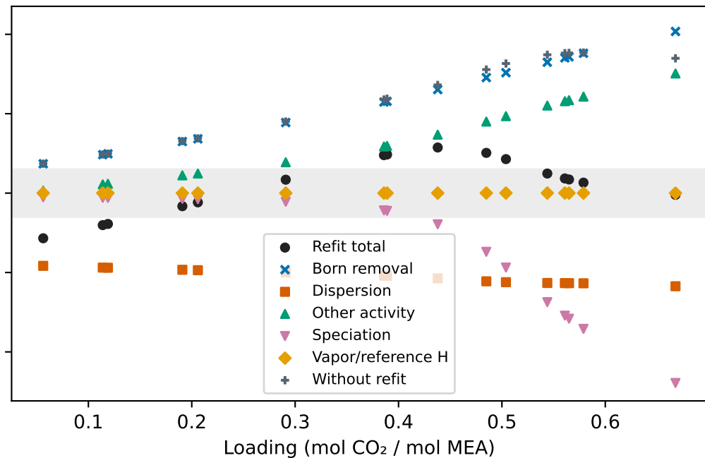
Born-off activity-sum shifts exceed speciation shifts Pipeline verification on pre-#152 data; method development, not manuscript values 313.15 K
