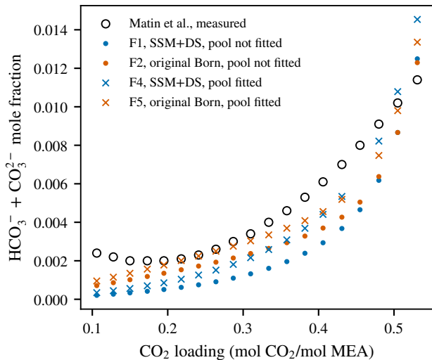
(a) Titration bicarbonate pool, 20 °C
