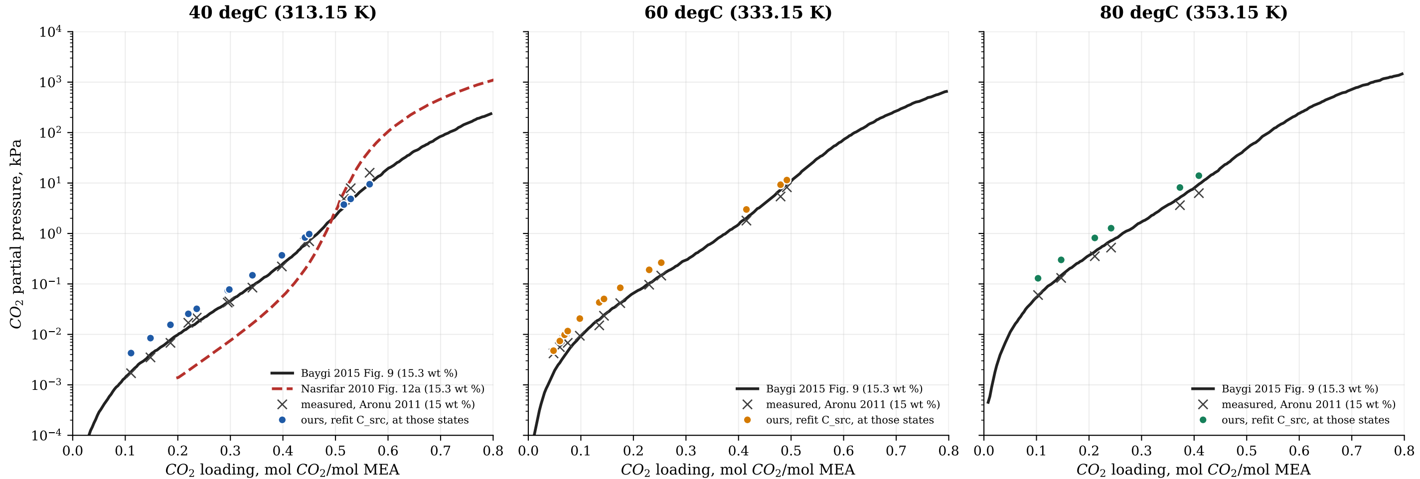
15 wt % MEA: published Baygi and Nasrifar model lines, and our refit C_src on the Aronu 2011 states
