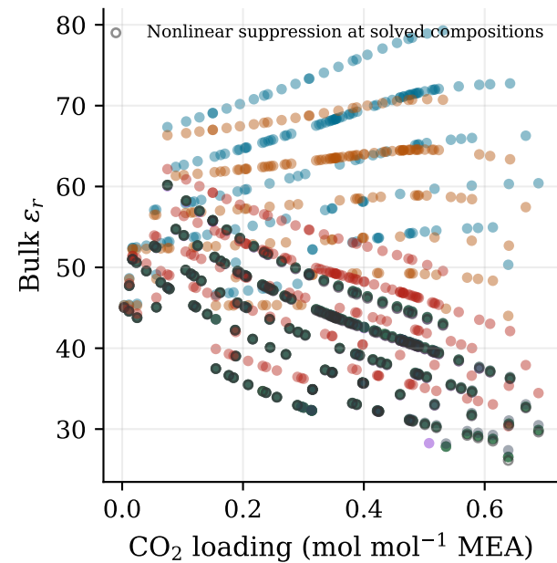
Permittivity response
