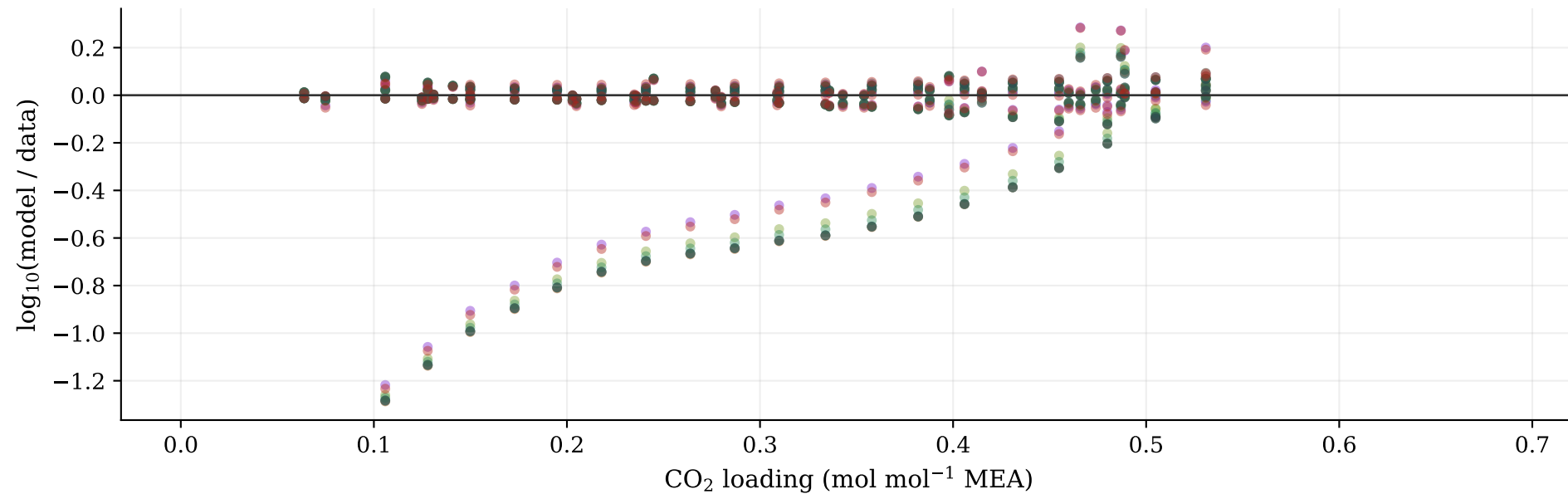
Speciation residuals
