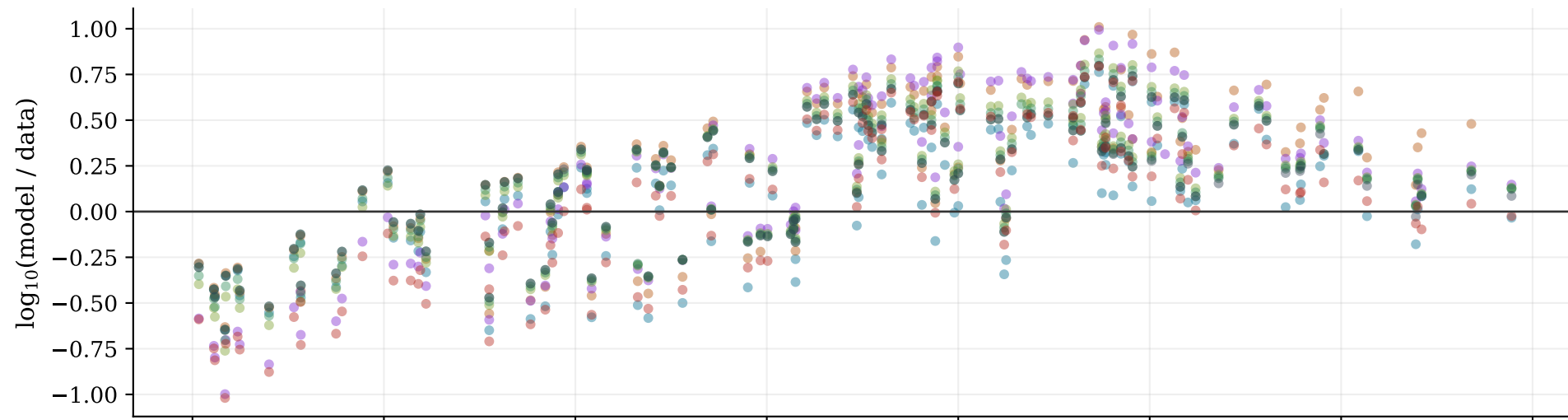
Speciation residuals
