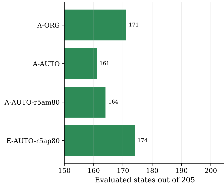
Numerical coverage
