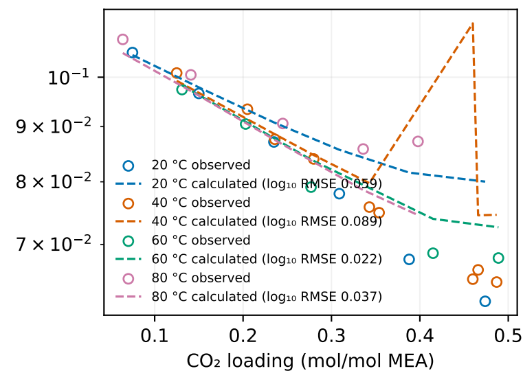
MEA + MEAH+
