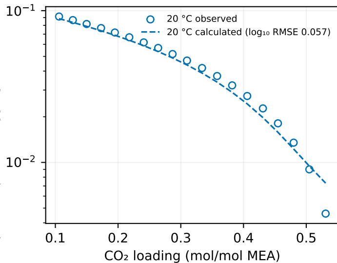
MEACOO-
