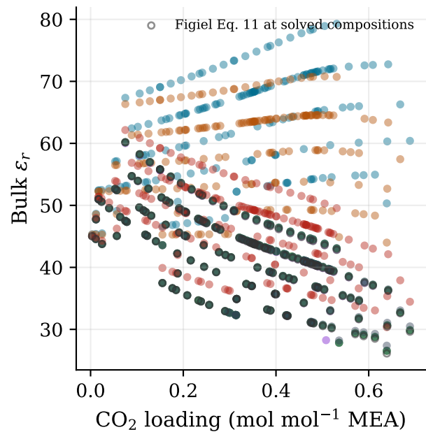
Permittivity response
