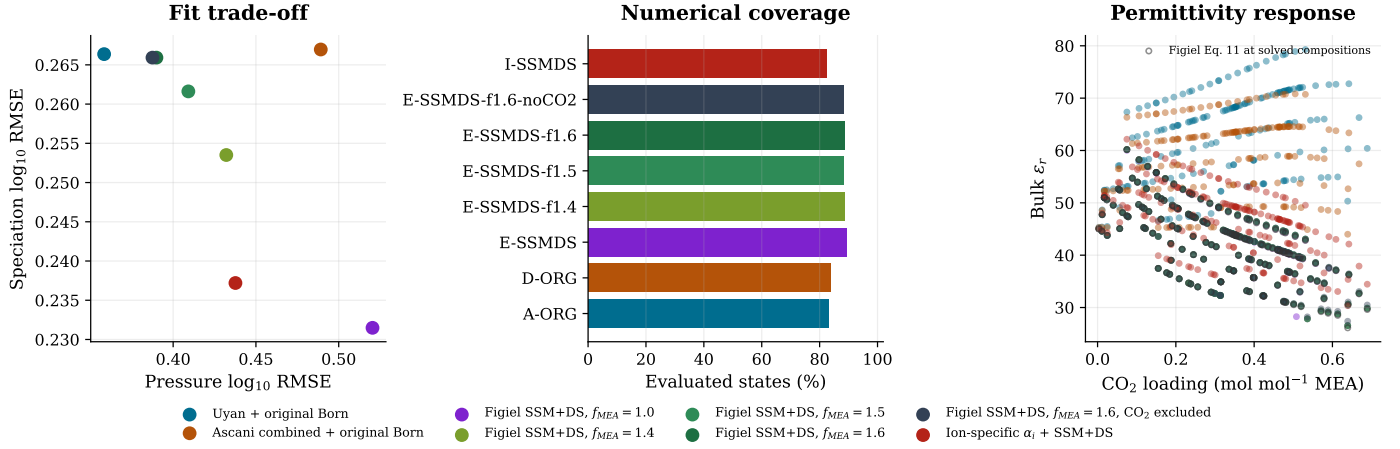
Fixed-parameter Born-permittivity comparison
