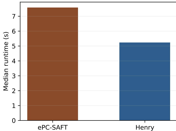
Accepted-row runtime
