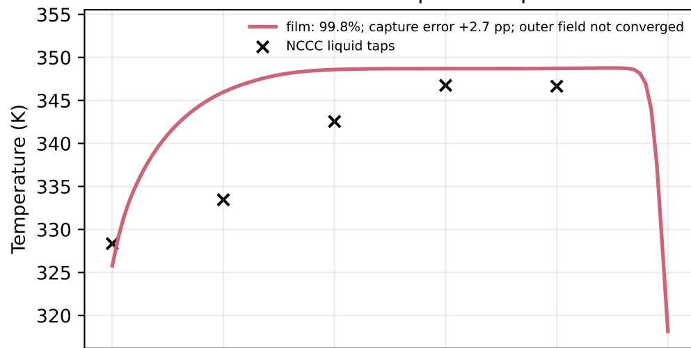
1C reactive-film temperature profile
