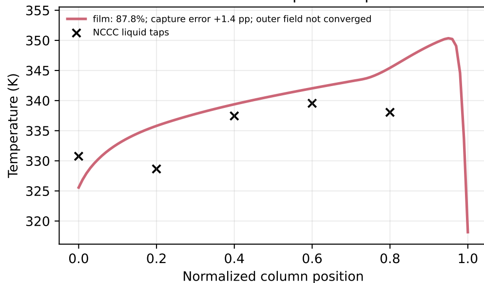
5C reactive-film temperature profile
