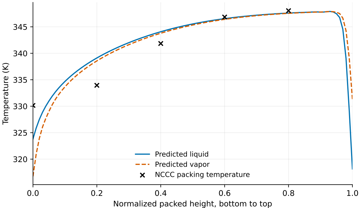
Case 3C: nine-species reactive ePC-SAFT
